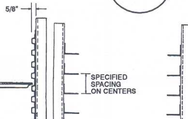
ANGLE LEDGE SUPPORT
