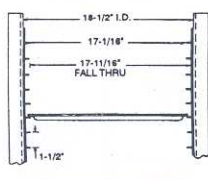
EXTRUDED SIDE PANELS
