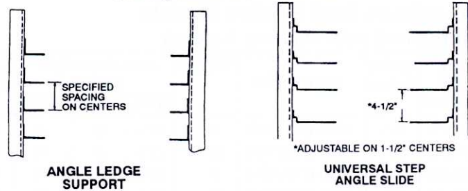
Angle Slide Type Nesting Racks MODEL 9589-N-12
